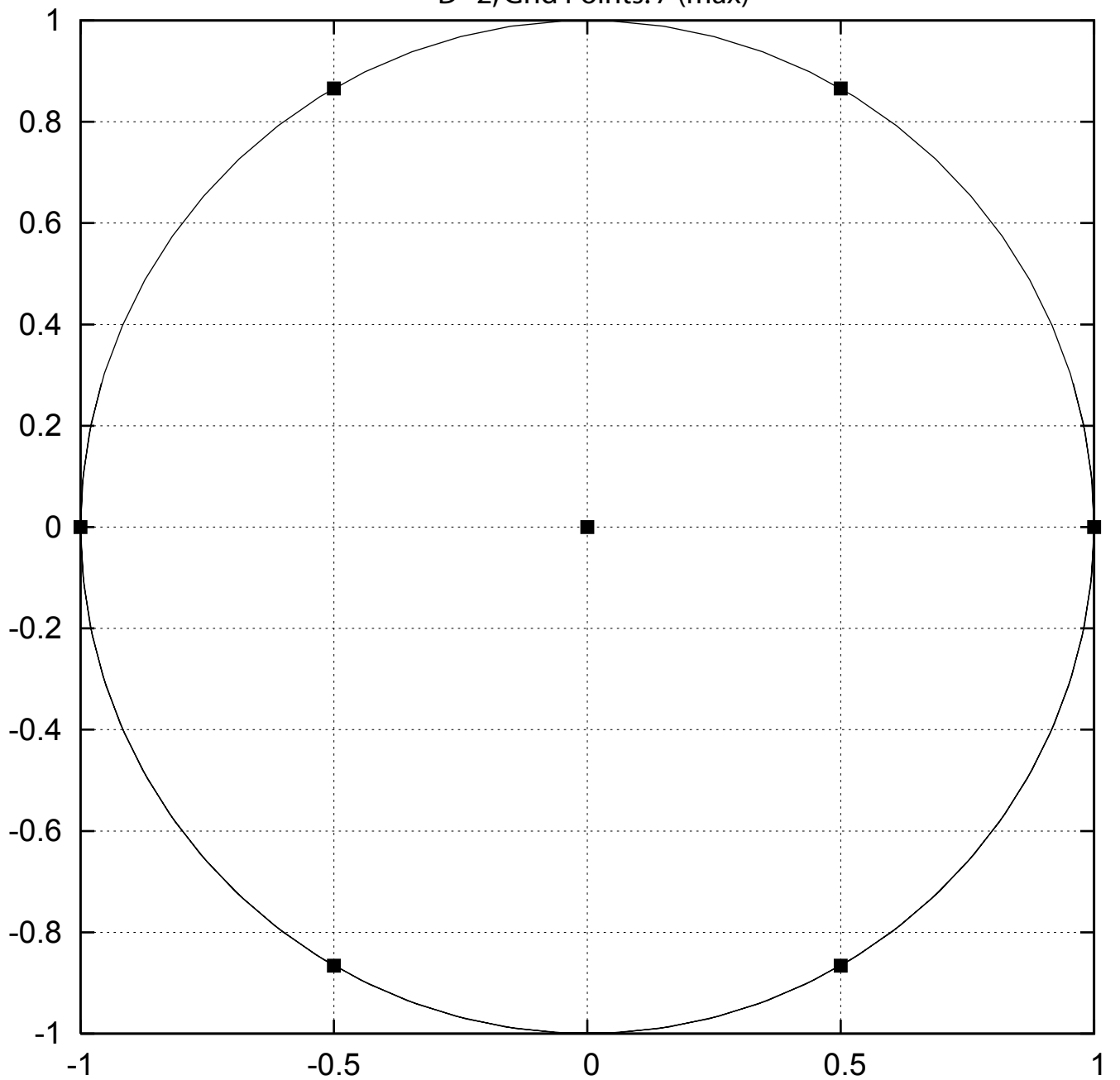
D=2, Grid Points: 7 (max)
