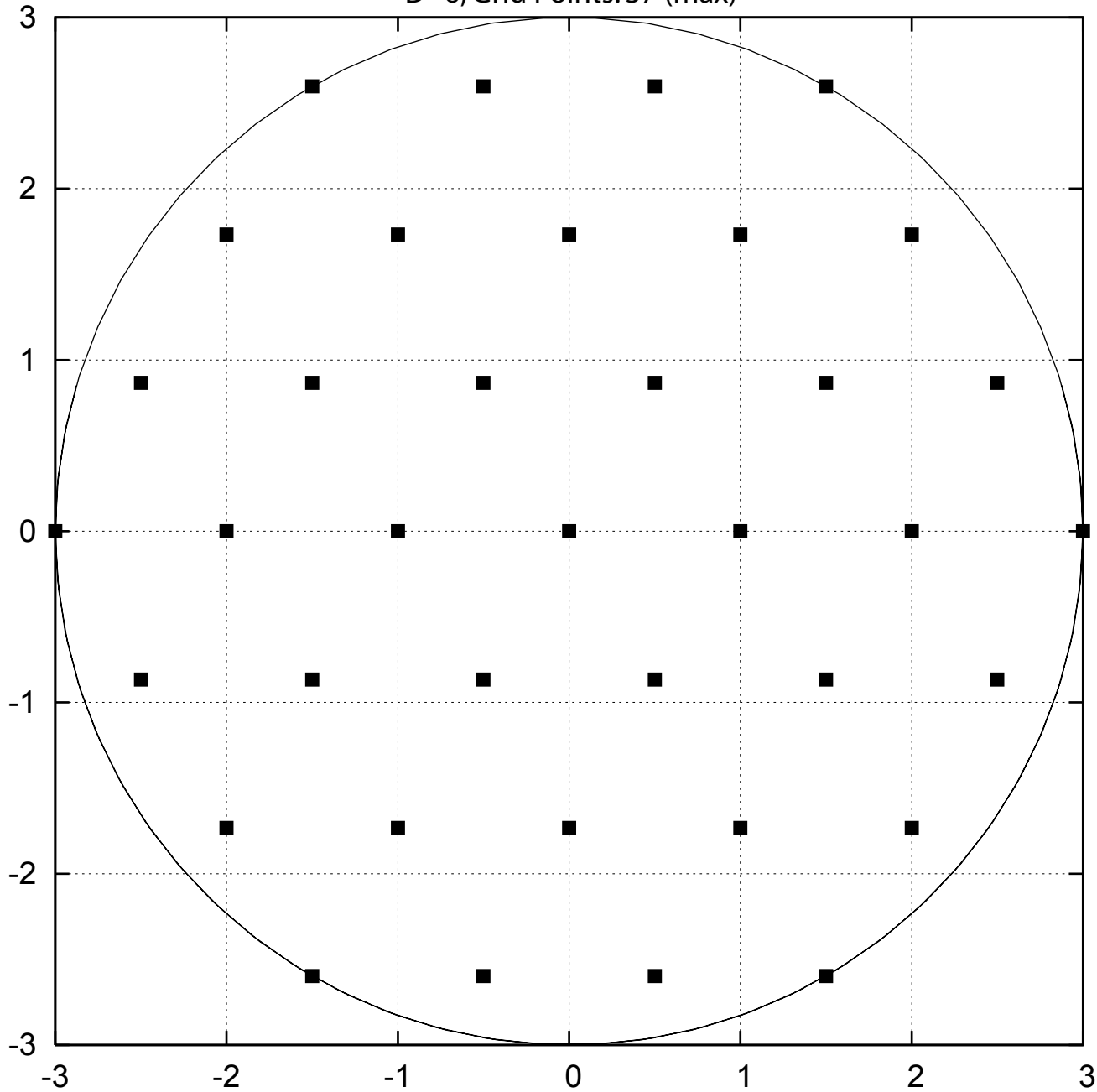
D=6, Grid Points: 37 (max)
