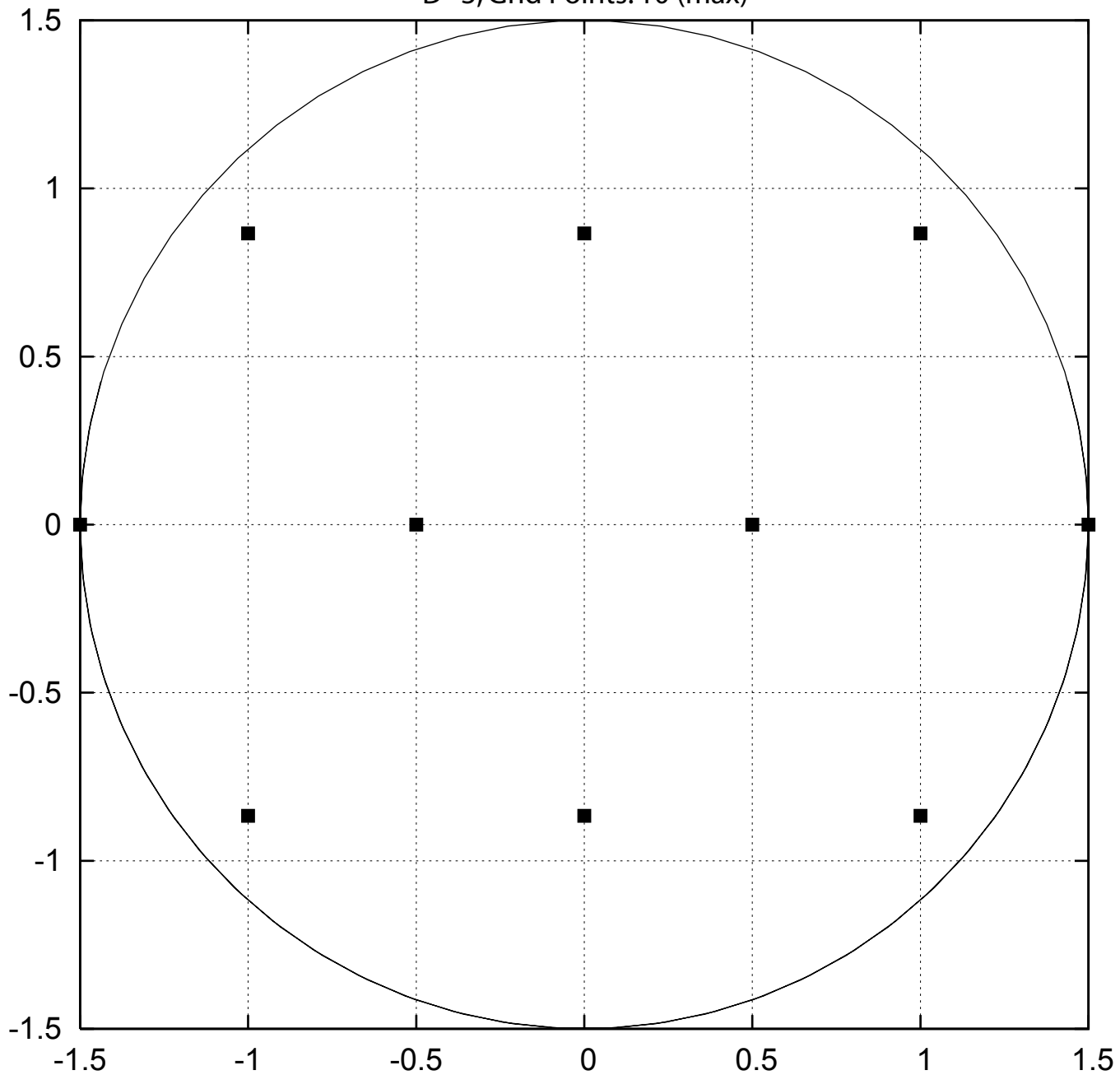
D=3, Grid Points: 10 (max)
