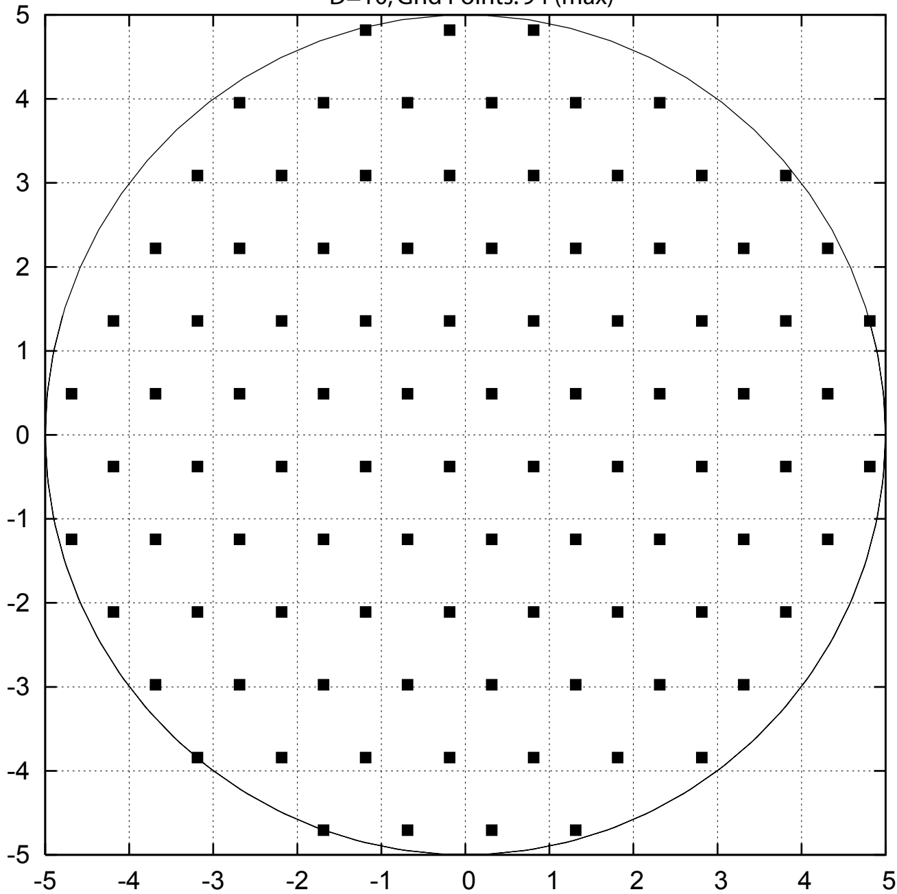
D=10, Grid Points: 94 (max)
