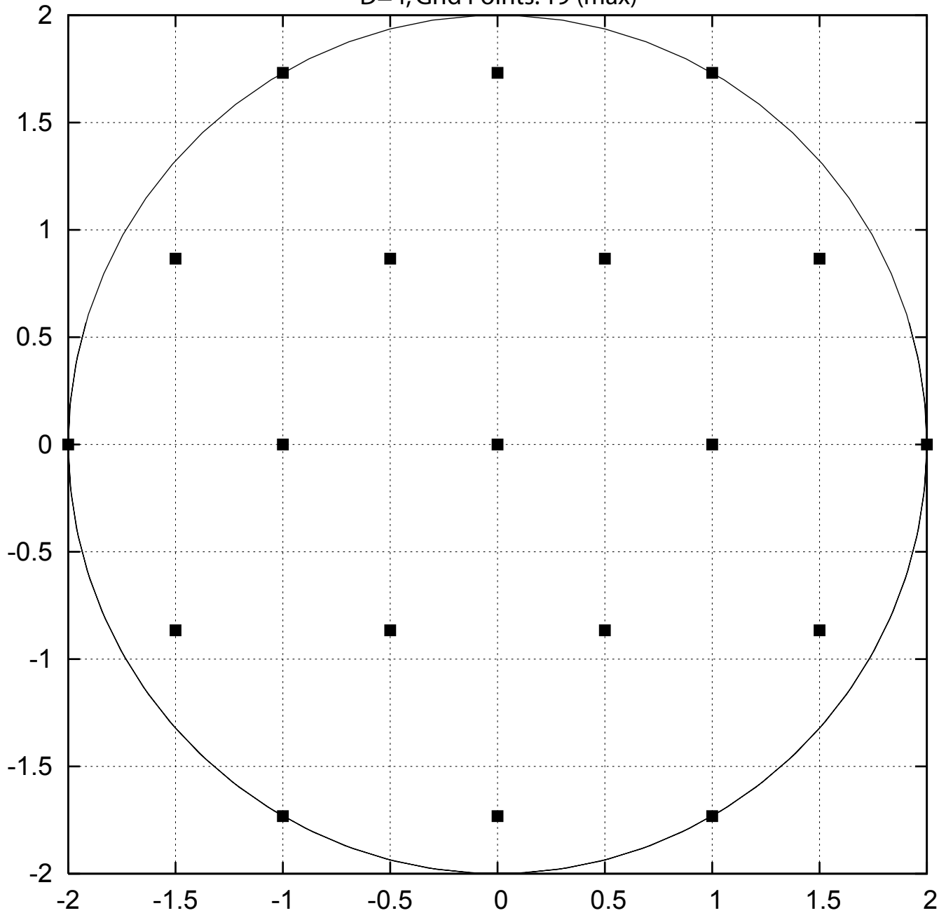
D=4, Grid Points: 19 (max)
