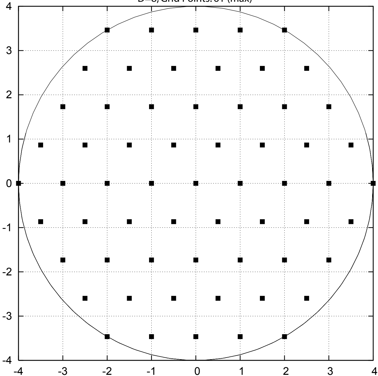
D=8, Grid Points: 61 (max)
