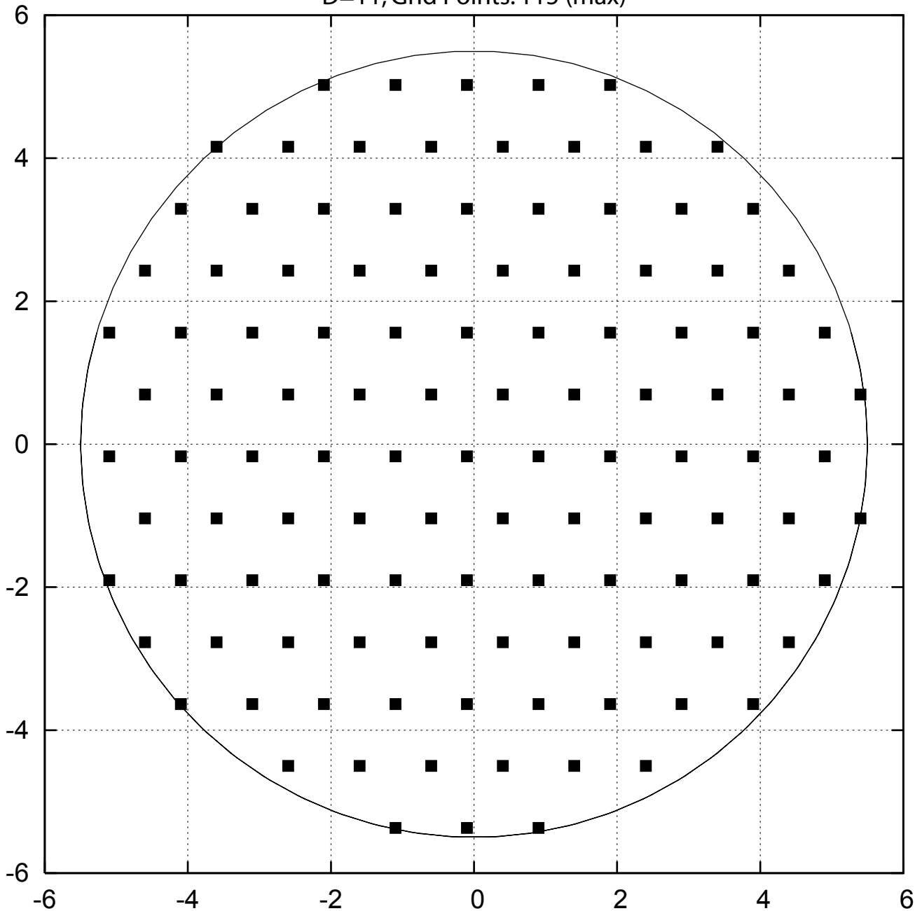
D=11, Grid Points: 115 (max)
