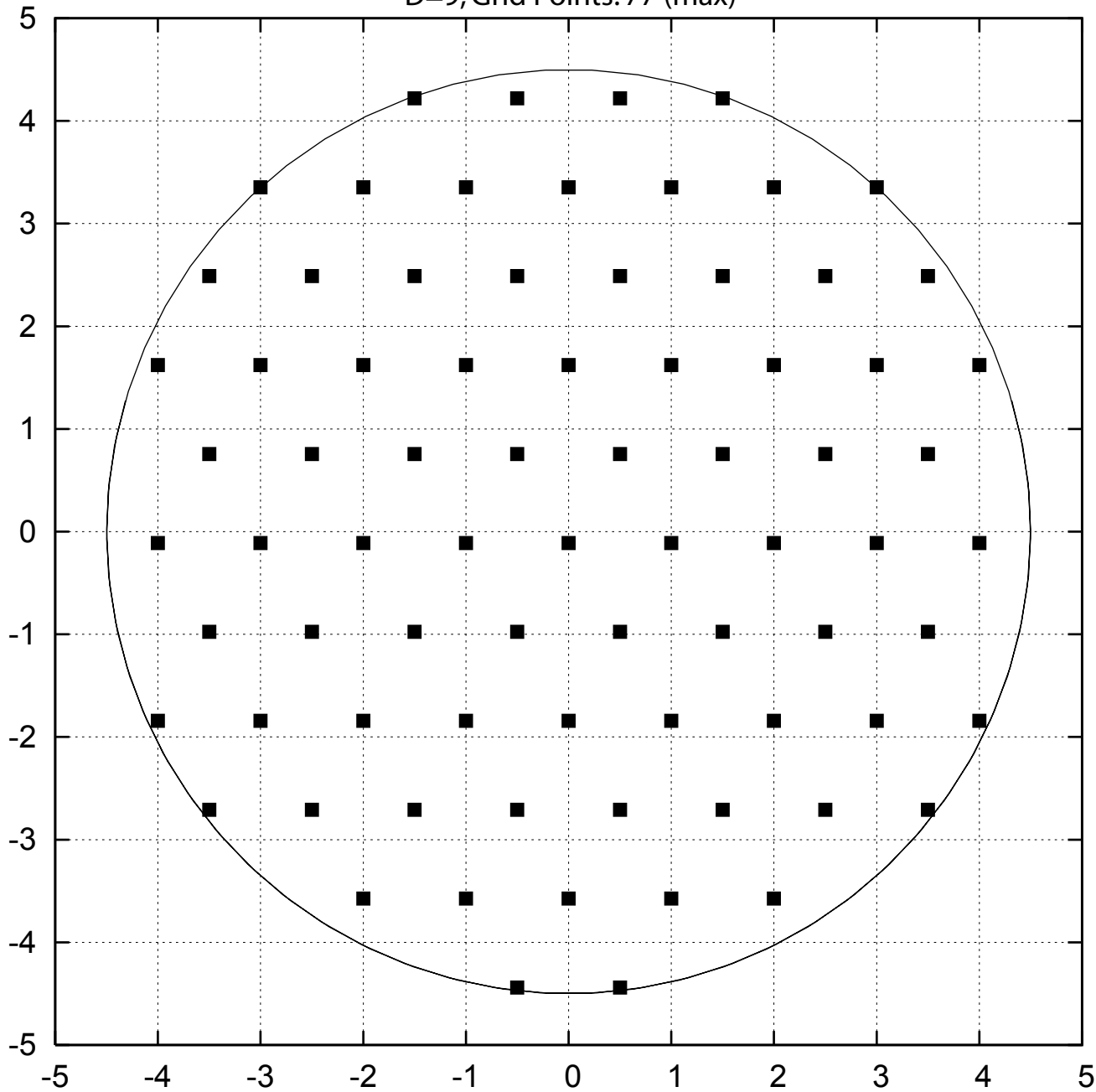
D=9, Grid Points: 77 (max)
