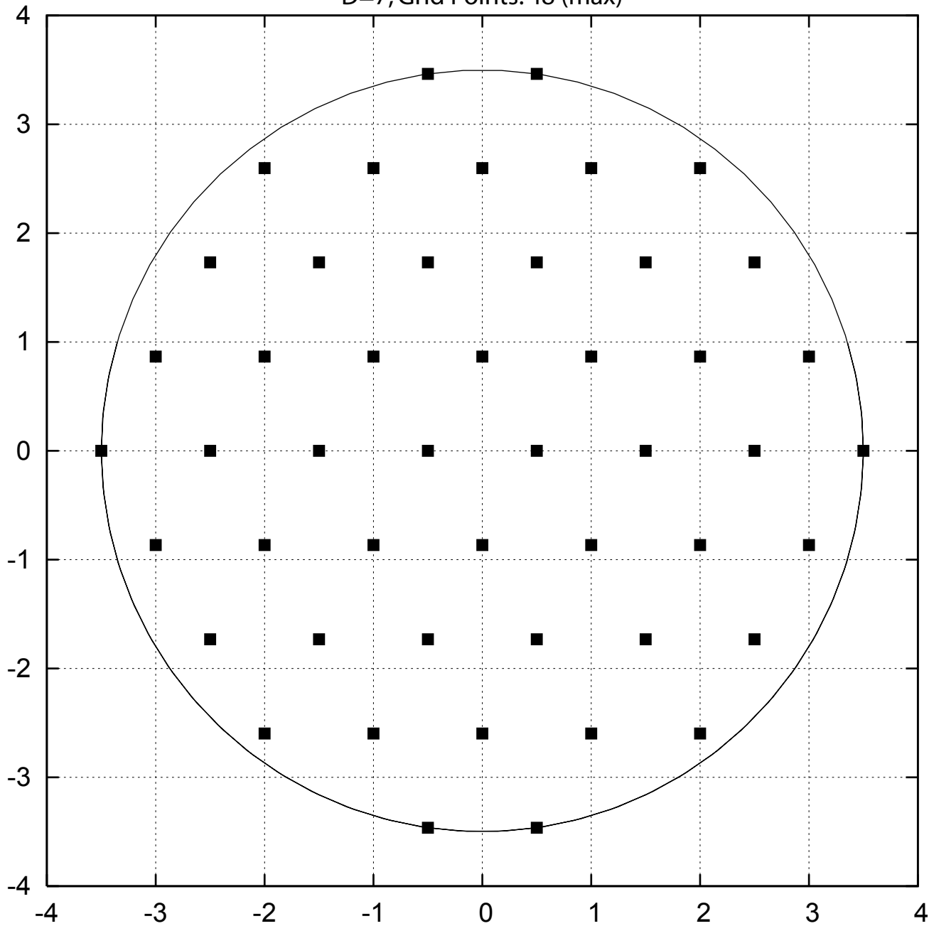
D=7, Grid Points: 48 (max)
