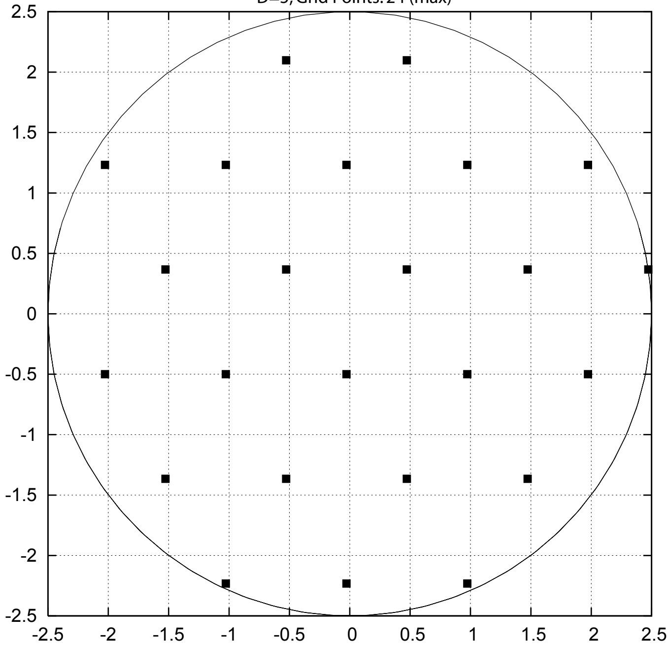
D=5, Grid Points: 24 (max)
