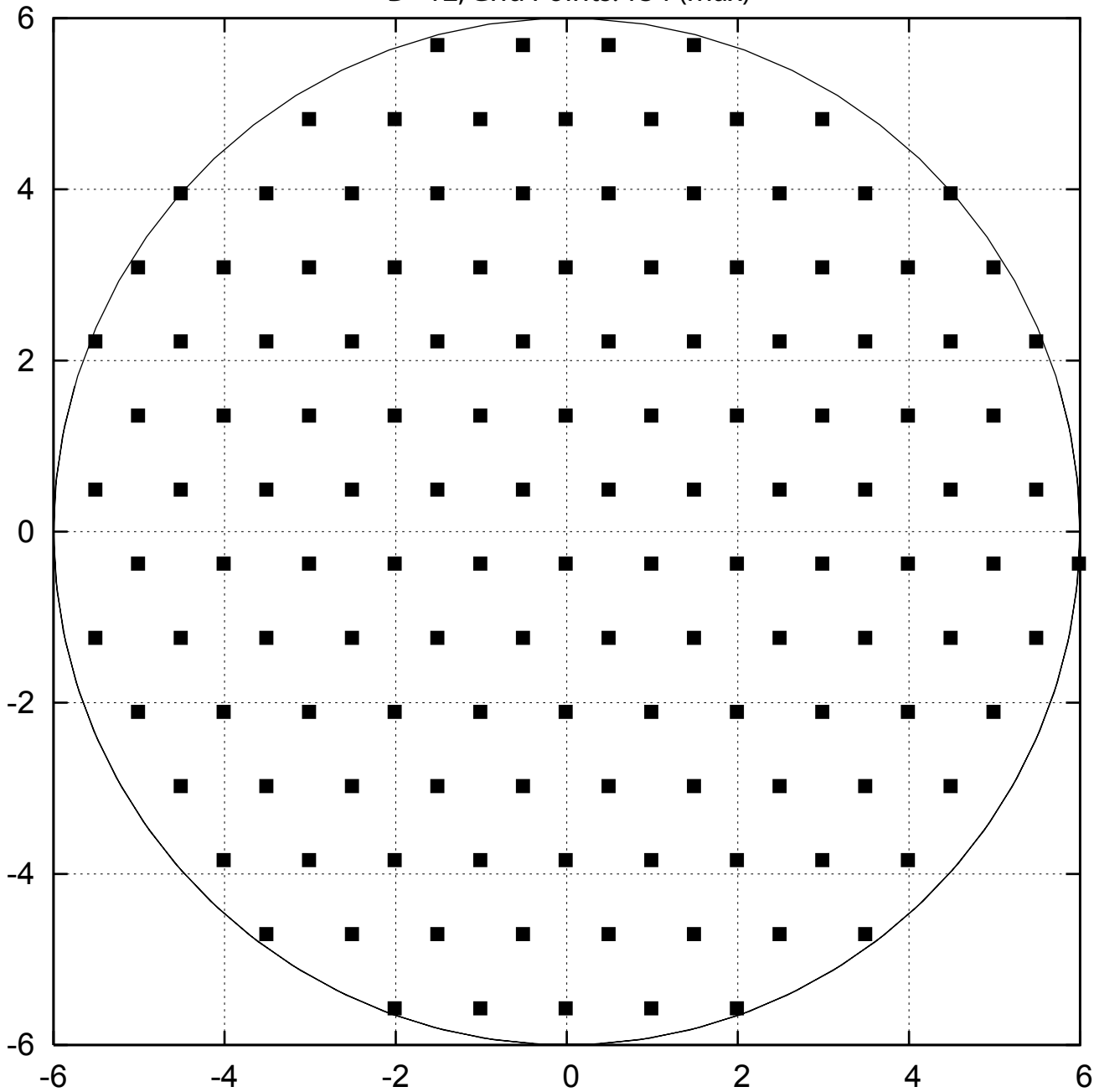
D=12, Grid Points: 134 (max)
