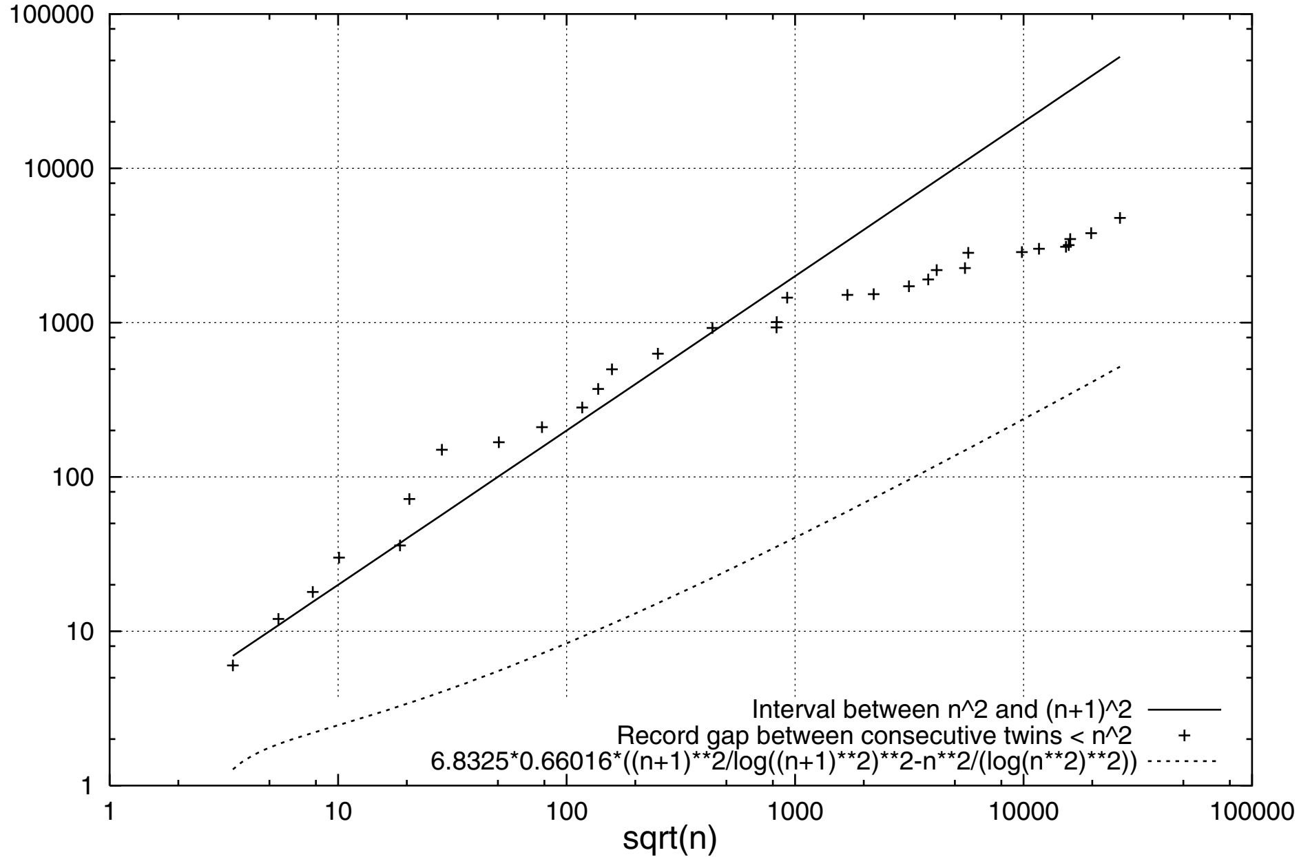
Comparison: Record gaps between twin primes and intervals between consecutive squares
