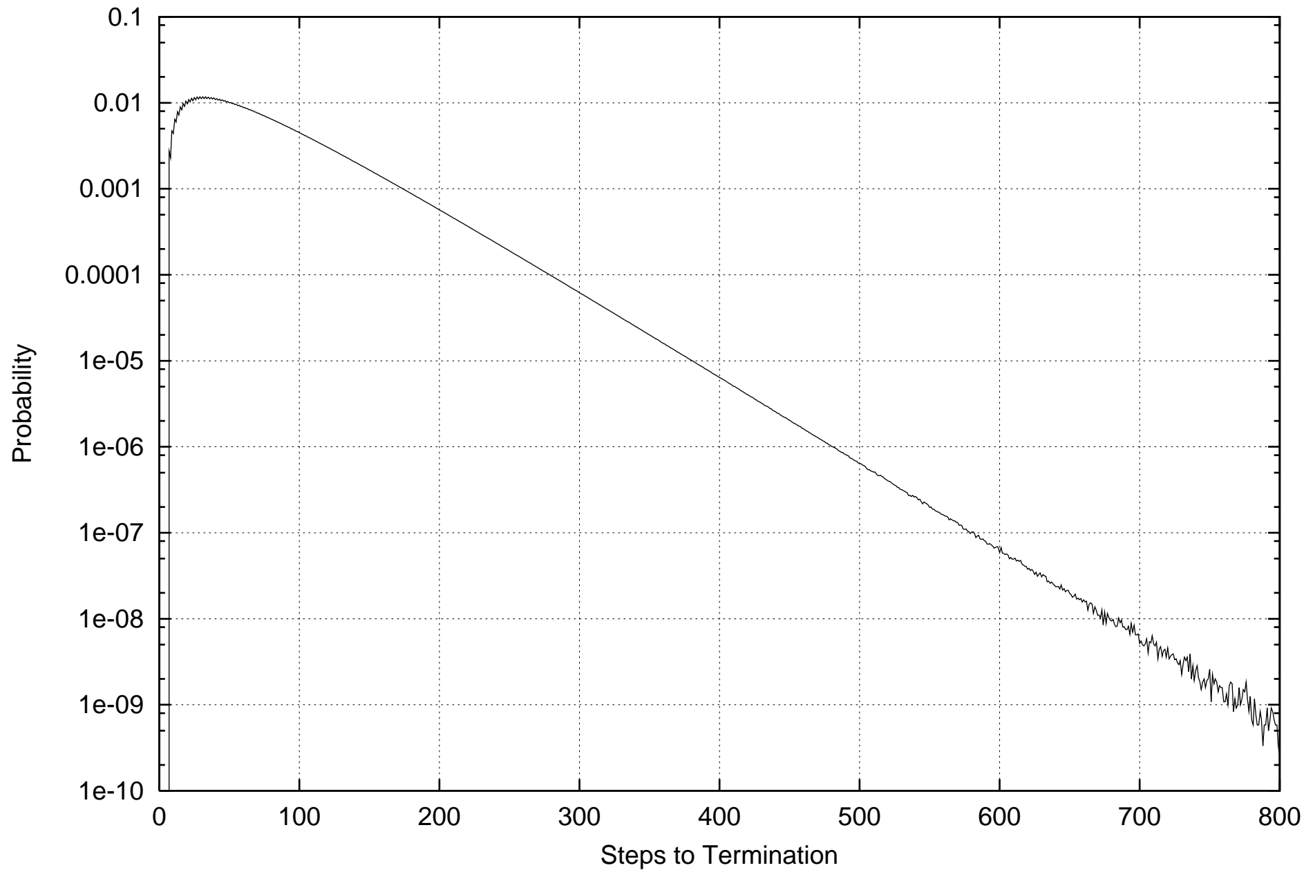
Self-Trapping Random Walk on 2-D Lattice ( 1.2 \cdot 10^{10} Walks)
