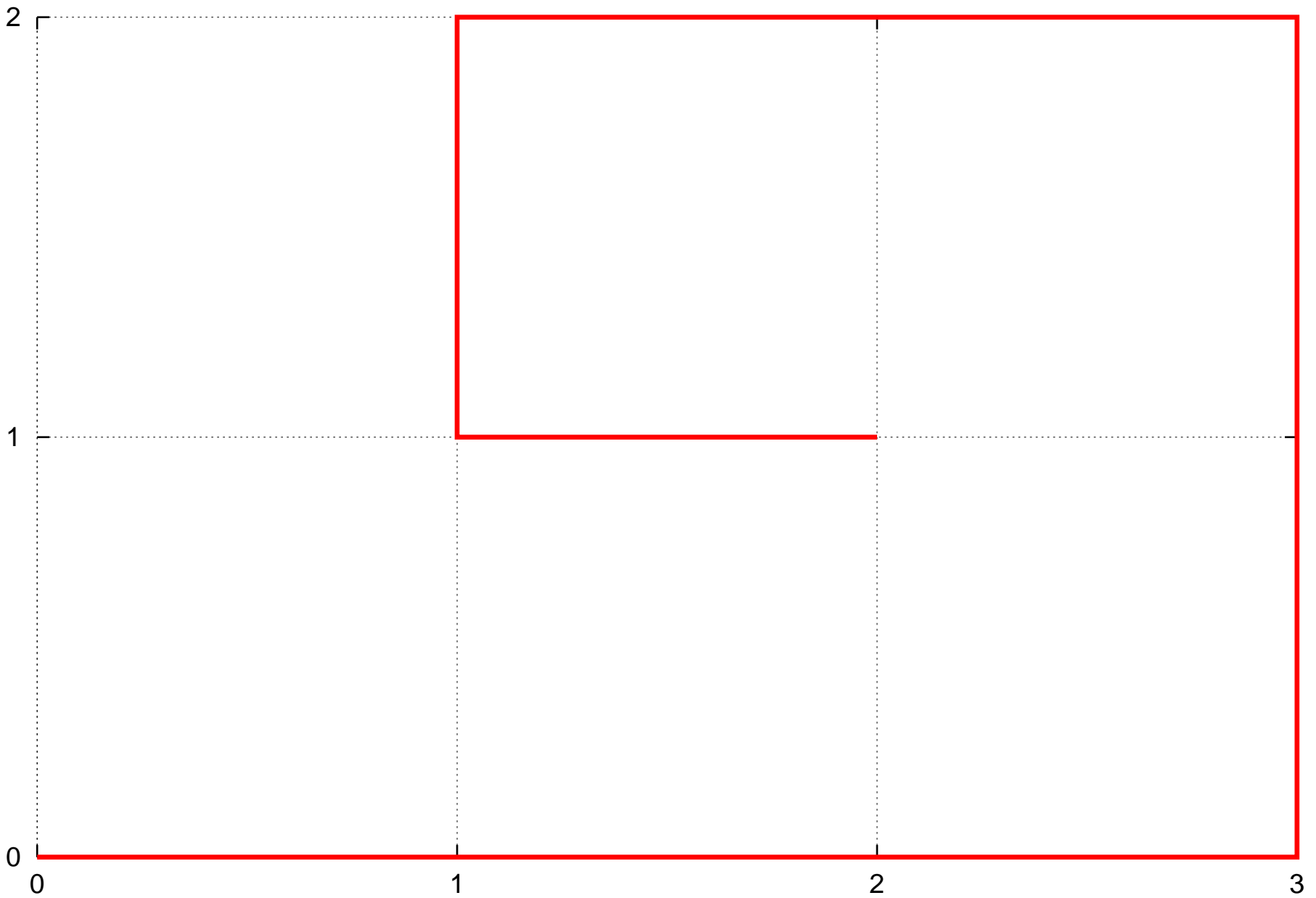
Walk n=9, 1 constrained step
