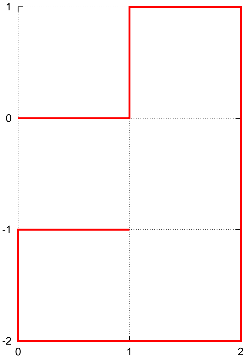
Maximally 2-constrained walks of length 10
