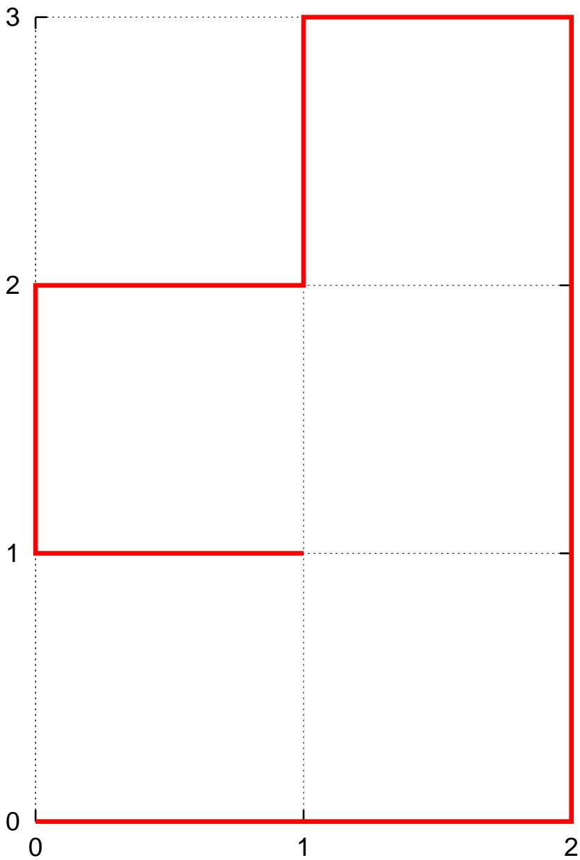
Maximally 2-constrained walks of length 10
