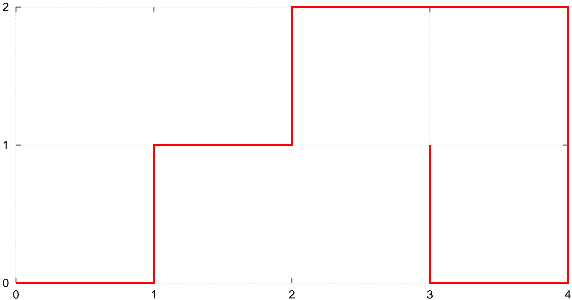
Unconstrained walks of length 10
