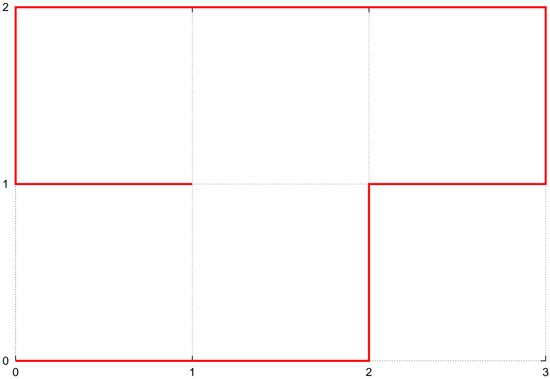
Maximally 2-constrained walks of length 10
