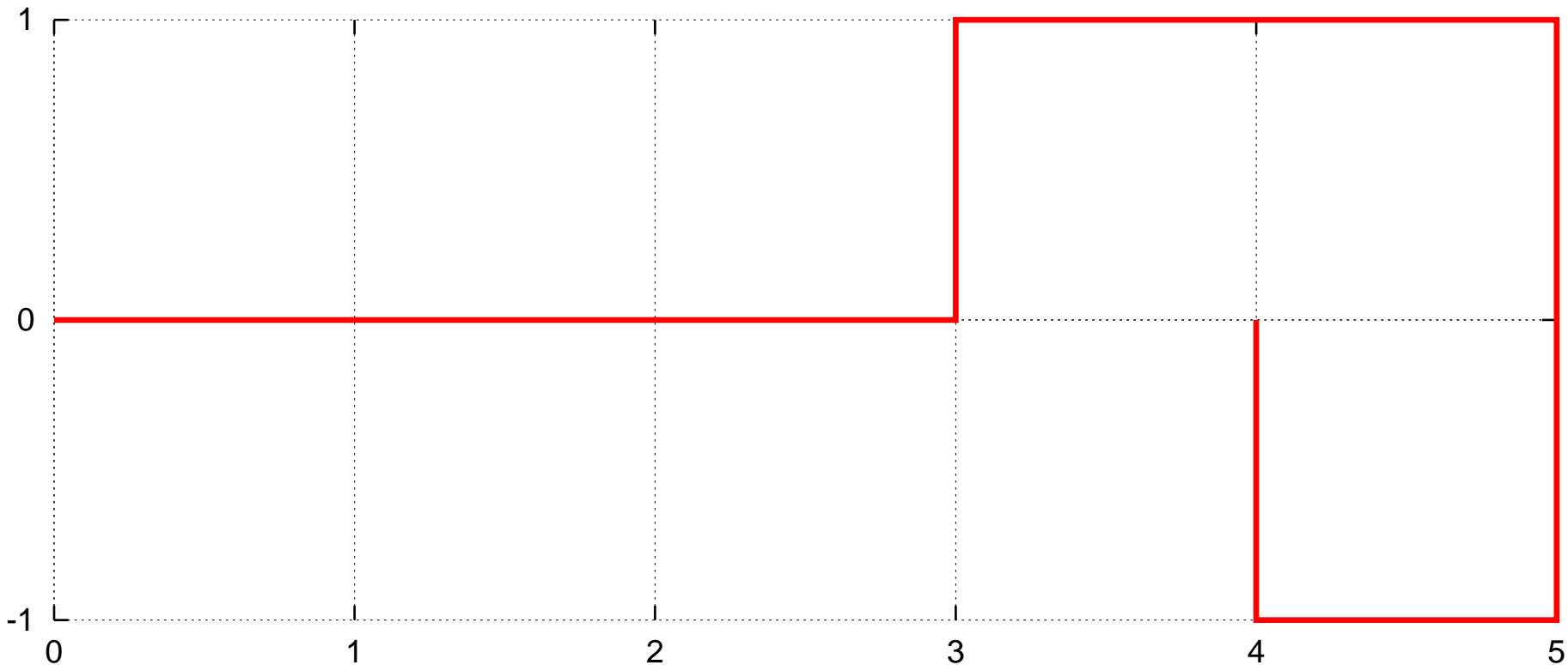
Unconstrained walks of length 10
