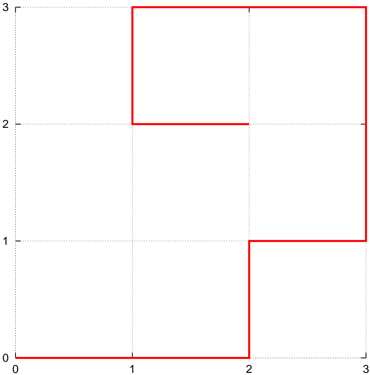
Unconstrained walks of length 10
