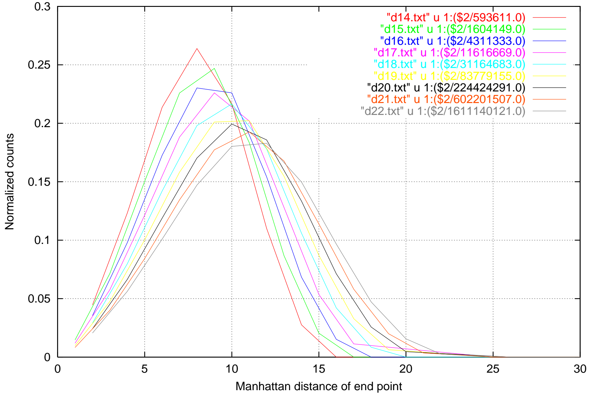
Manhattan Distance Start-End for n-step SAWs
