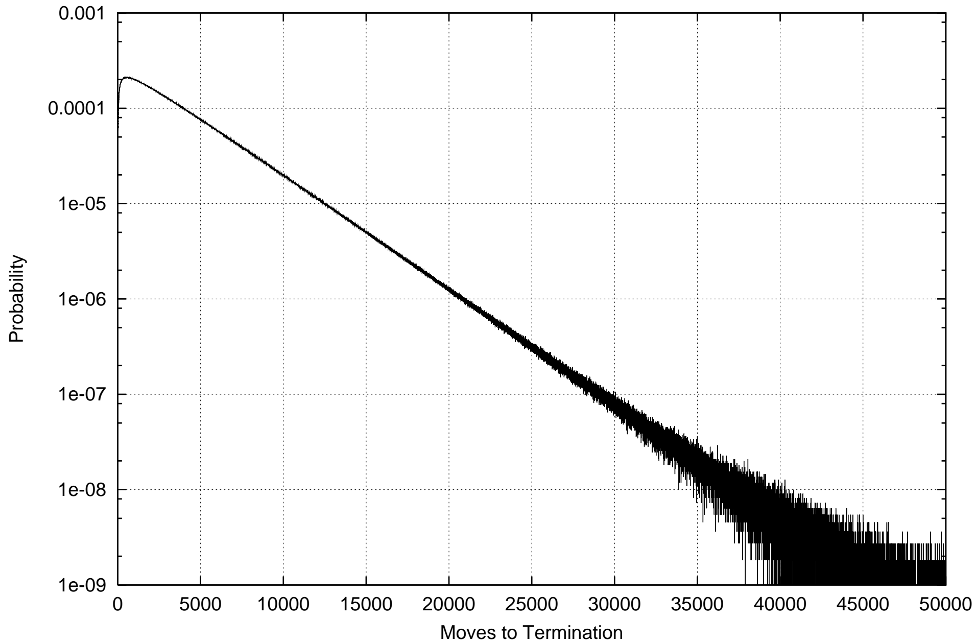
Self-Trapping Random Walk on 3-D Lattice ( 1.1 \cdot 10^9 Walks)
