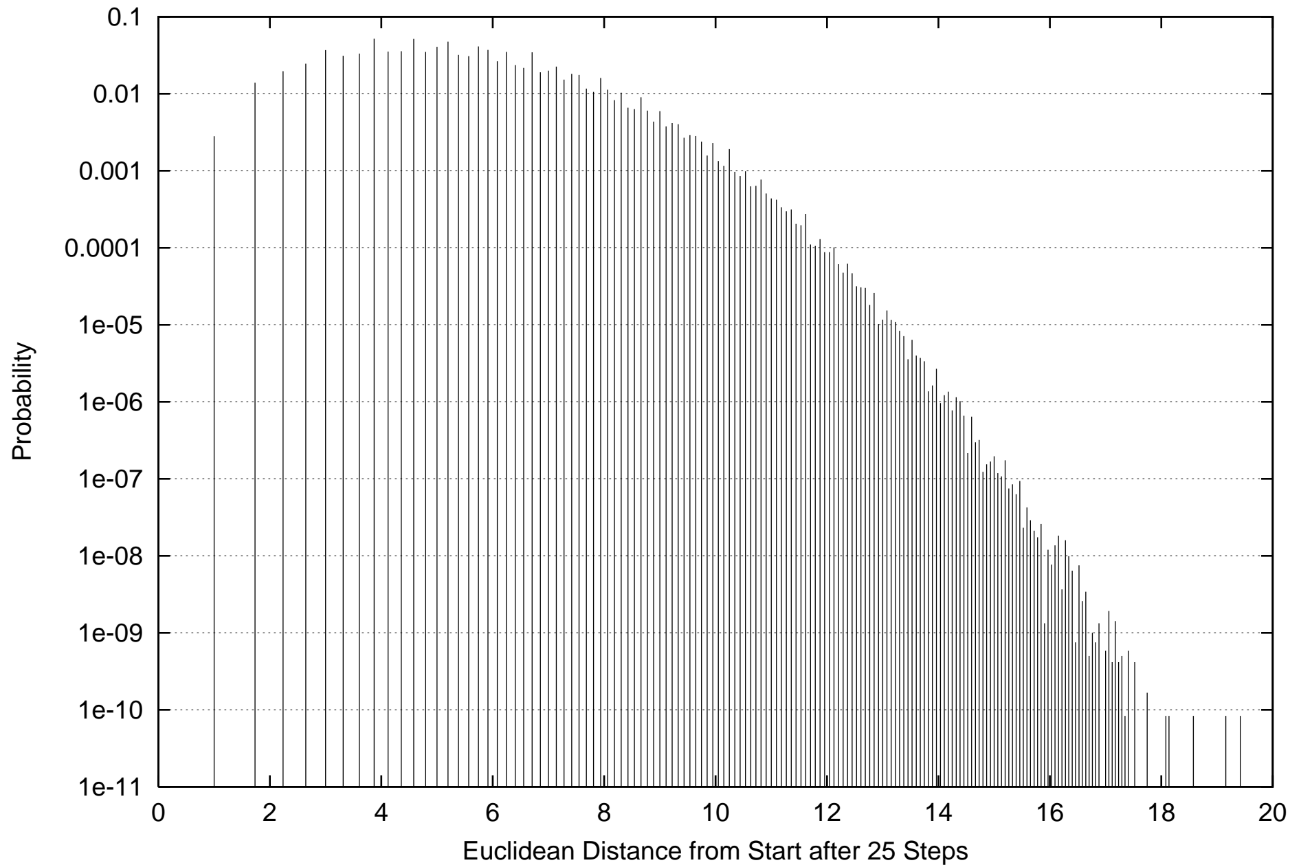
1.2*10 10 Self-Trapping Random Walks on 4-D Lattice
